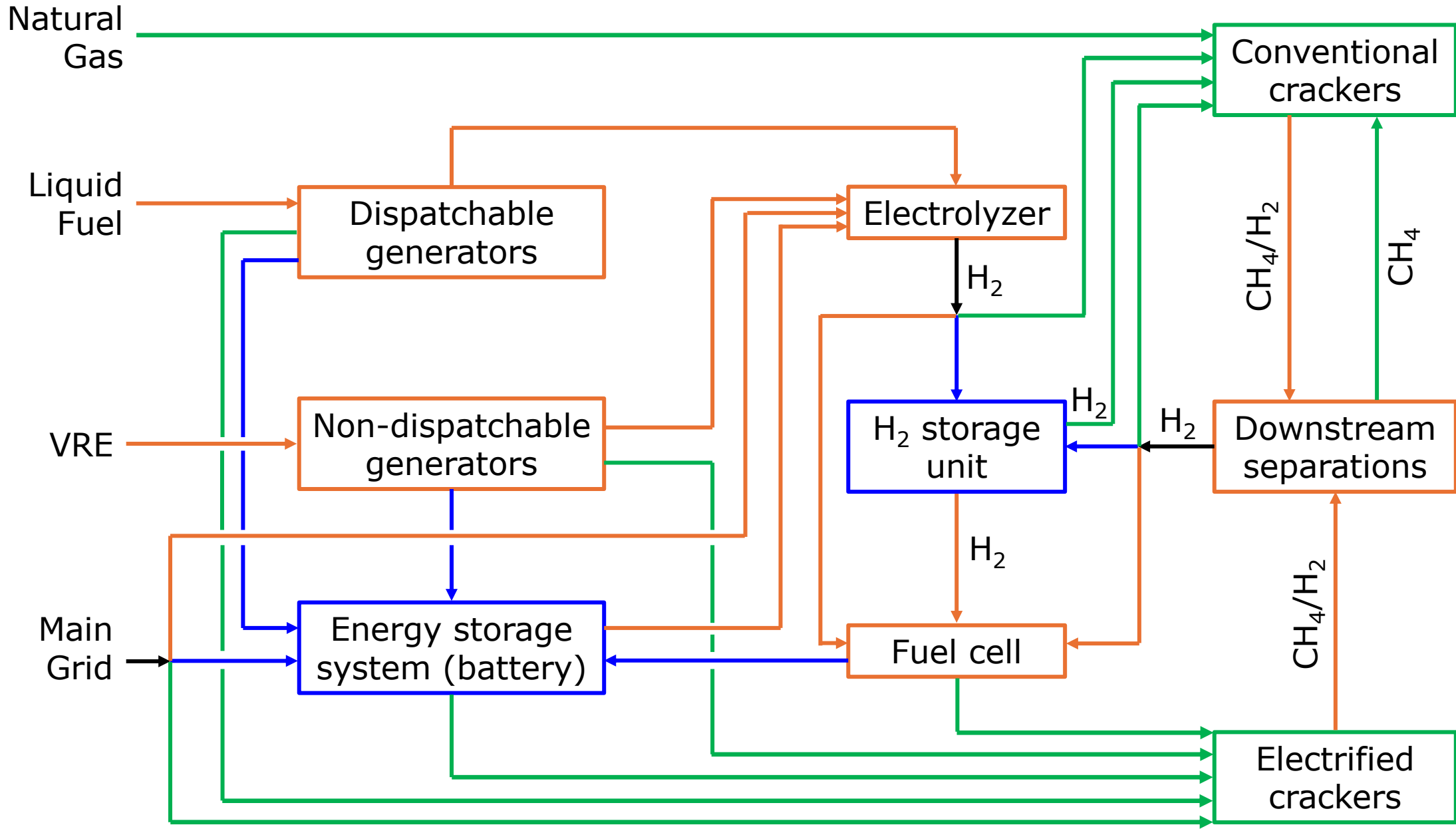
Connections & unit operations associated with: ■ Energy conversion ■ Energy storage ■ Energy usage
